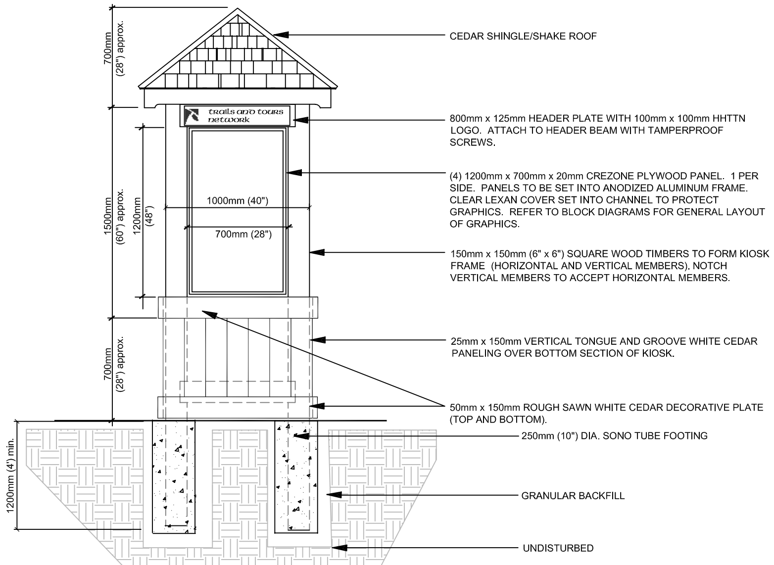
4 SIDED TRAILHEAD KIOSK: ELEVATION (MAJOR STAGING AREA)
